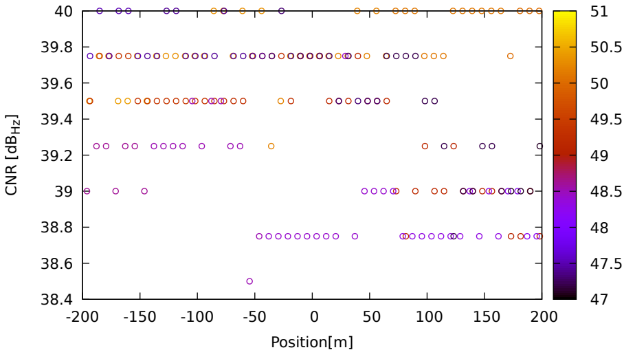
CNR vs position for G01 (L5) on XiaomiMi8 - DOY 262 jam. 2
