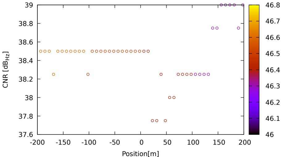
CNR vs position for G01 (L5) on XiaomiMi8 - DOY 262 jam. 3
