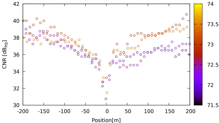
CNR vs position for G03 (L1) on XiaomiMi8 - DOY 262 jam. 1
