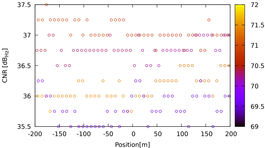
CNR vs position for G03 (L5) on XiaomiMi8 - DOY 262 jam. 2
