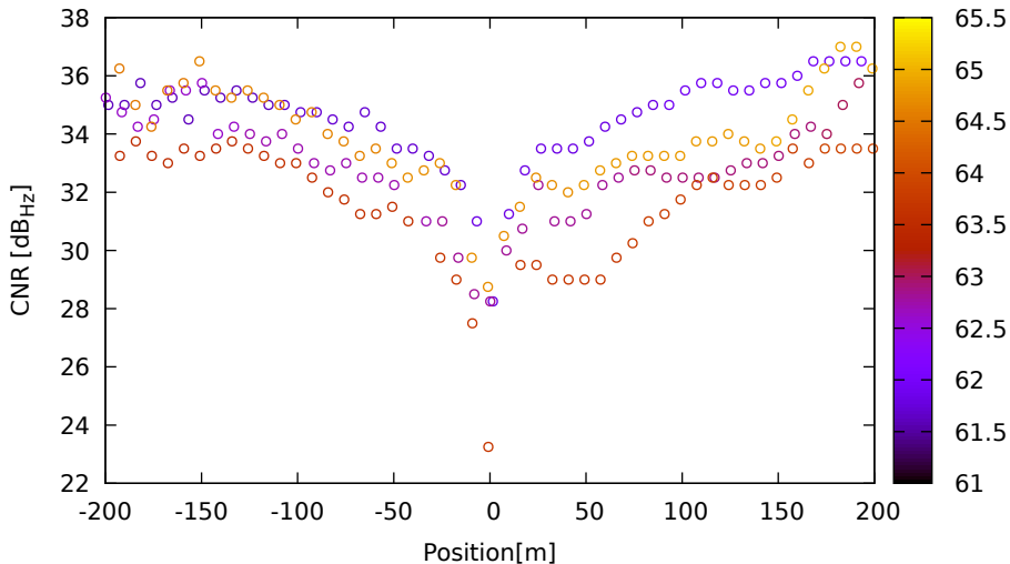
CNR vs position for G04 (L1) on XiaomiMi8 - DOY 262 jam. 1
