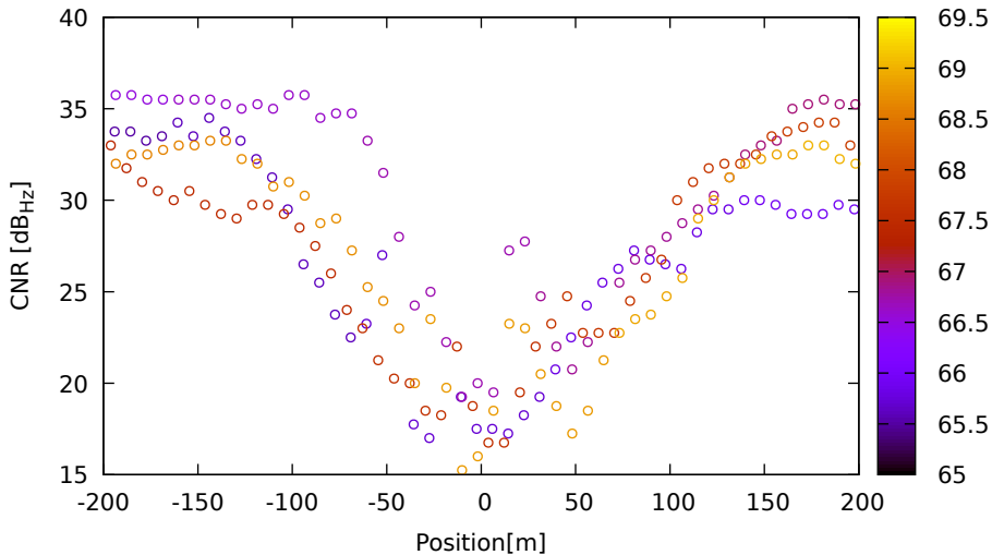
CNR vs position for G04 (L1) on XiaomiMi8 - DOY 262 jam. 2
