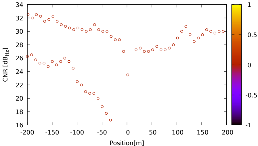
CNR vs position for G06 (L1) on XiaomiMi8 - DOY 262 jam. 1
