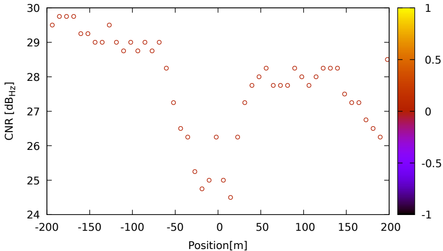
CNR vs position for G06 (L1) on XiaomiMi8 - DOY 262 jam. 3
