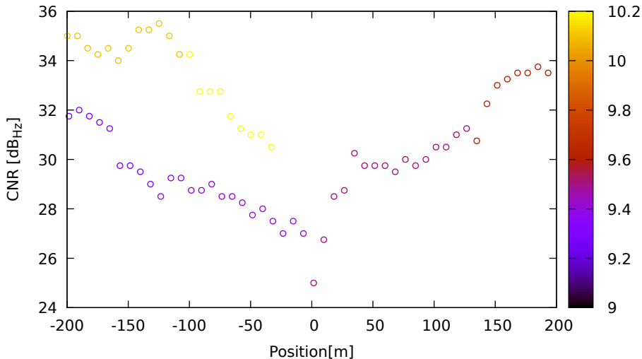
CNR vs position for G06 (L5) on XiaomiMi8 - DOY 262 jam. 1
