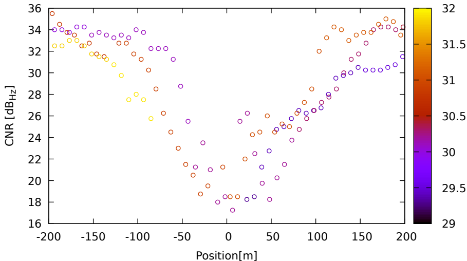
CNR vs position for G09 (L1) on XiaomiMi8 - DOY 262 jam. 2
