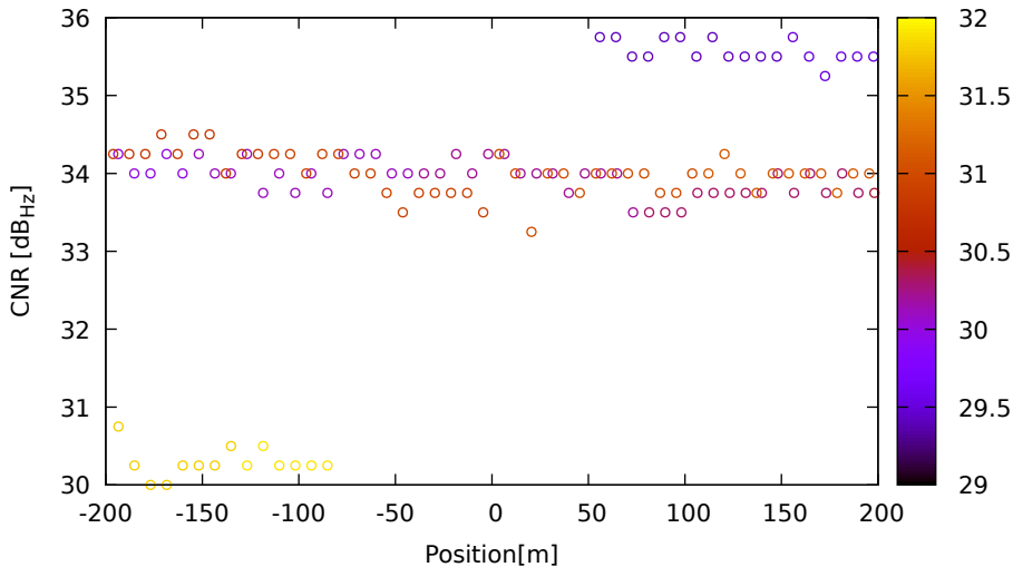
CNR vs position for G09 (L5) on XiaomiMi8 - DOY 262 jam. 2
