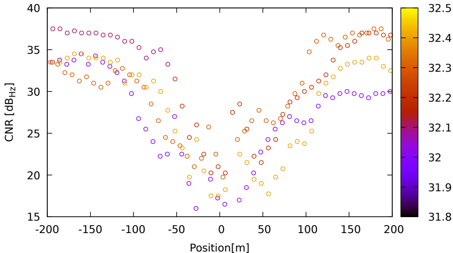
CNR vs position for G19 (L1) on XiaomiMi8 - DOY 262 jam. 2
