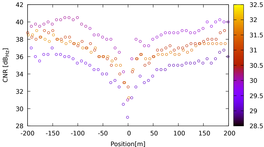
CNR vs position for G21 (L1) on XiaomiMi8 - DOY 262 jam. 1
