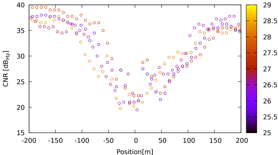
CNR vs position for G21 (L1) on XiaomiMi8 - DOY 262 jam. 2
