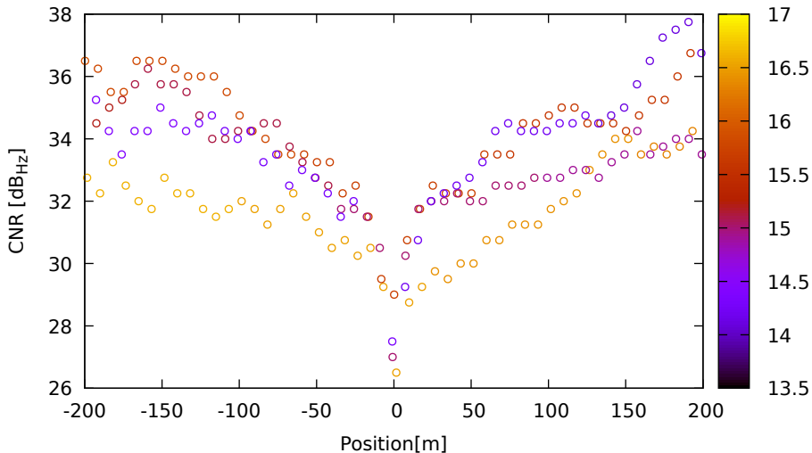
CNR vs position for G22 (L1) on XiaomiMi8 - DOY 262 jam. 1
