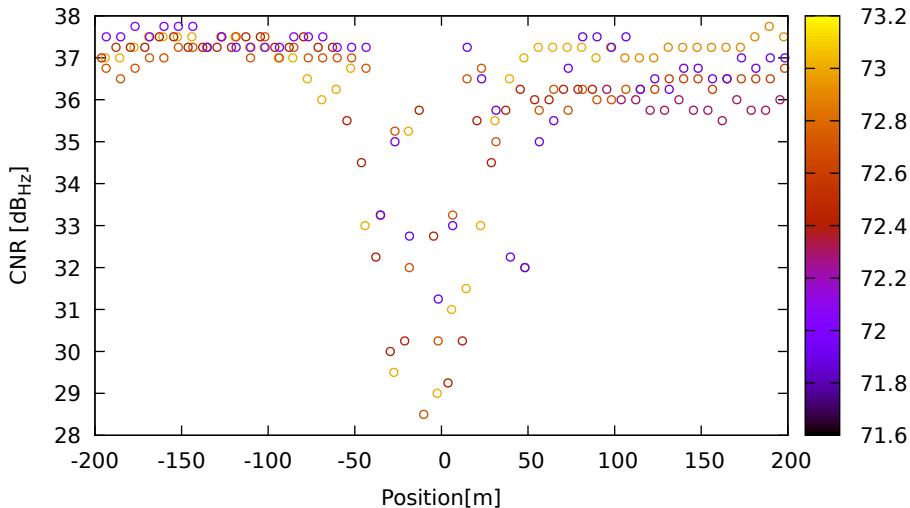
CNR vs position for R01 (G1) on XiaomiMi8 - DOY 262 jam. 2
