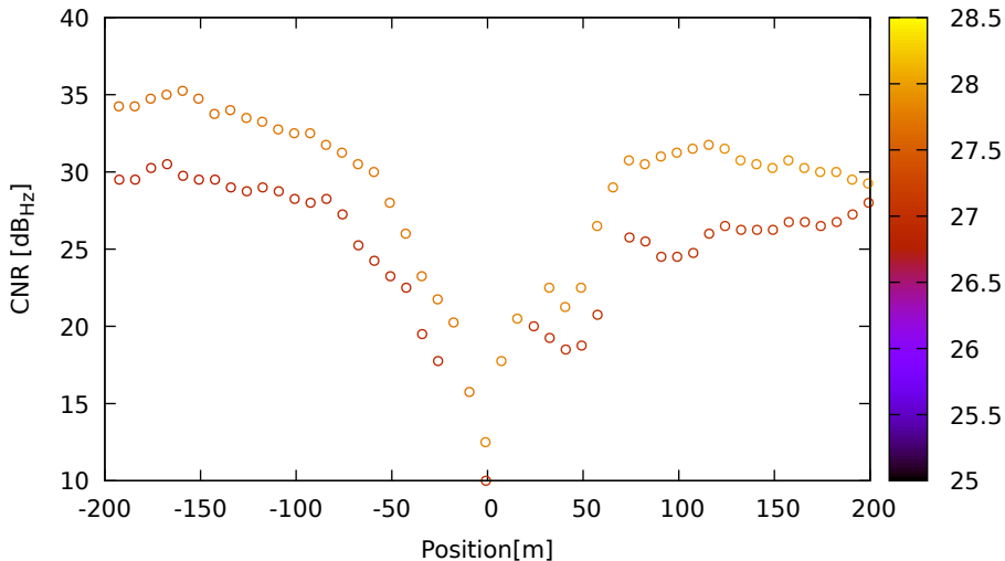
CNR vs position for R02 (G1) on XiaomiMi8 - DOY 262 jam. 1
