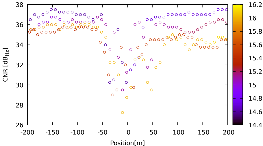
CNR vs position for R10 (G1) on XiaomiMi8 - DOY 262 jam. 2
