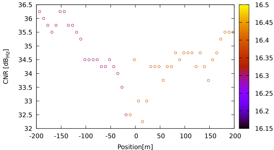
CNR vs position for R10 (G1) on XiaomiMi8 - DOY 262 jam. 3
