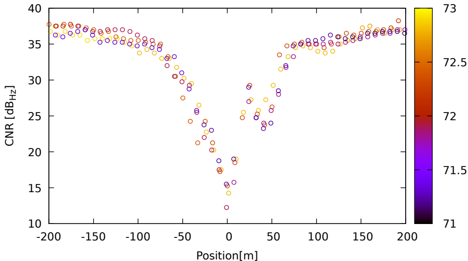
CNR vs position for R24 (G1) on XiaomiMi8 - DOY 262 jam. 1
