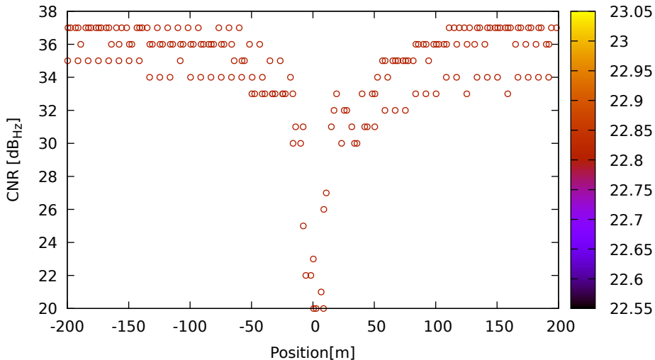
CNR vs position for C05 (B1) on HuaweiP40 - DOY 263 jam. 1
