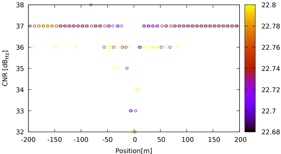
CNR vs position for C05 (B1) on HuaweiP40 - DOY 263 jam. 2
