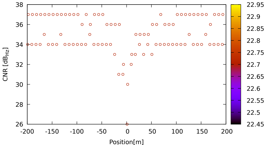
CNR vs position for C05 (B1) on HuaweiP40 - DOY 263 jam. 3
