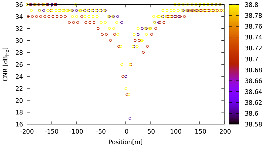
CNR vs position for C09 (B1) on HuaweiP40 - DOY 263 jam. 1
