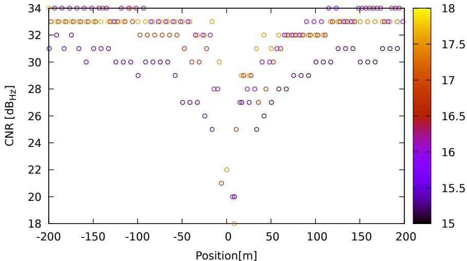
CNR vs position for C12 (B1) on HuaweiP40 - DOY 263 jam. 1
