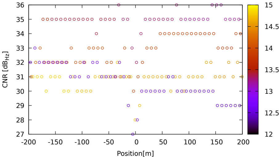
CNR vs position for C12 (B1) on HuaweiP40 - DOY 263 jam. 2
