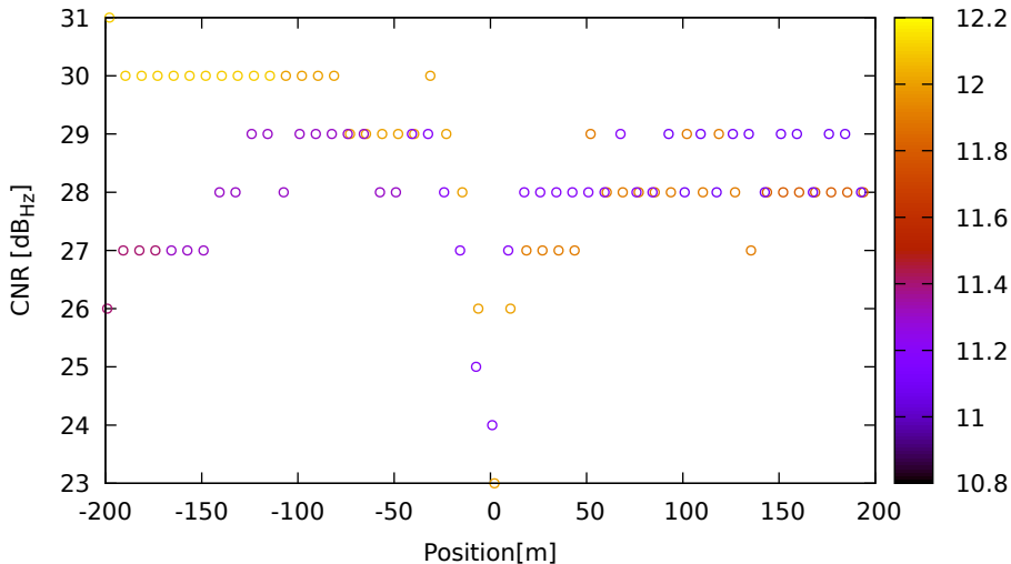
CNR vs position for C12 (B1) on HuaweiP40 - DOY 263 jam. 3
