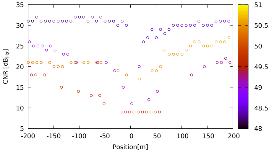
CNR vs position for C14 (B1) on HuaweiP40 - DOY 263 jam. 1
