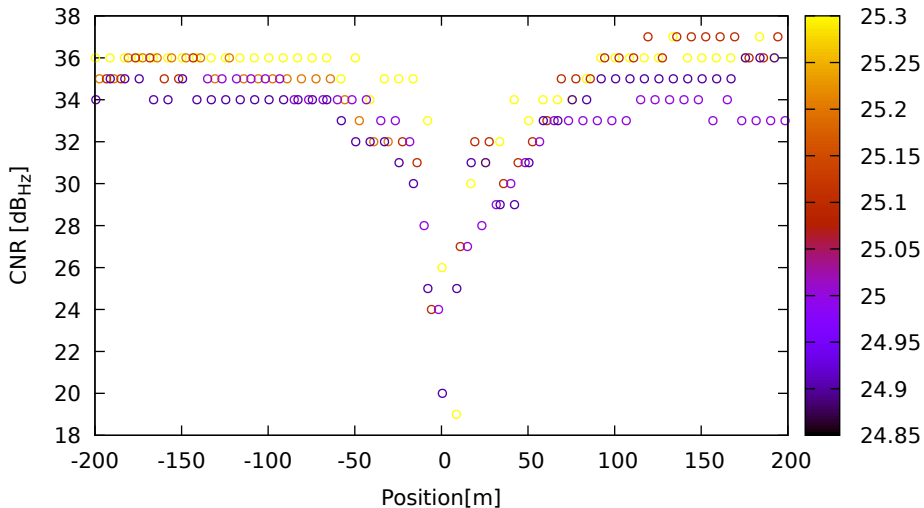
CNR vs position for C16 (B1) on HuaweiP40 - DOY 263 jam. 1
