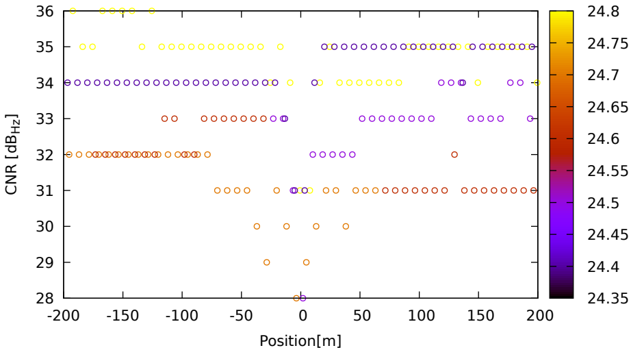
CNR vs position for C16 (B1) on HuaweiP40 - DOY 263 jam. 2
