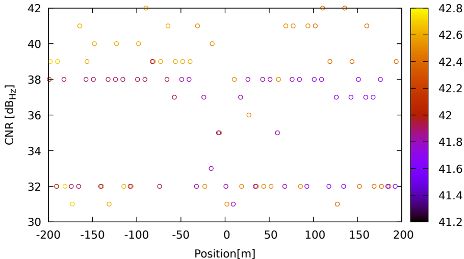
CNR vs position for C21 (B1) on HuaweiP40 - DOY 263 jam. 3
