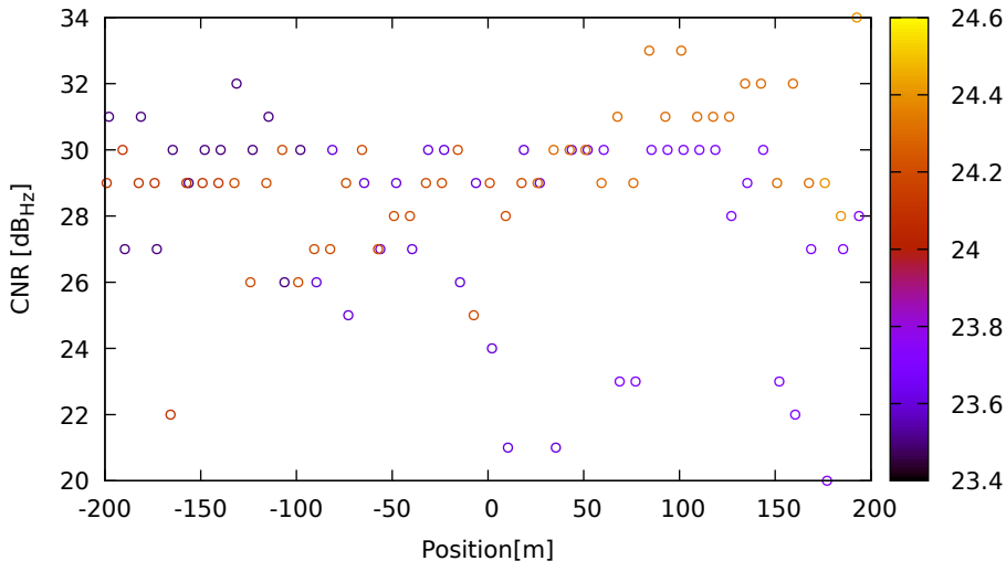
CNR vs position for C28 (B1) on HuaweiP40 - DOY 263 jam. 3
