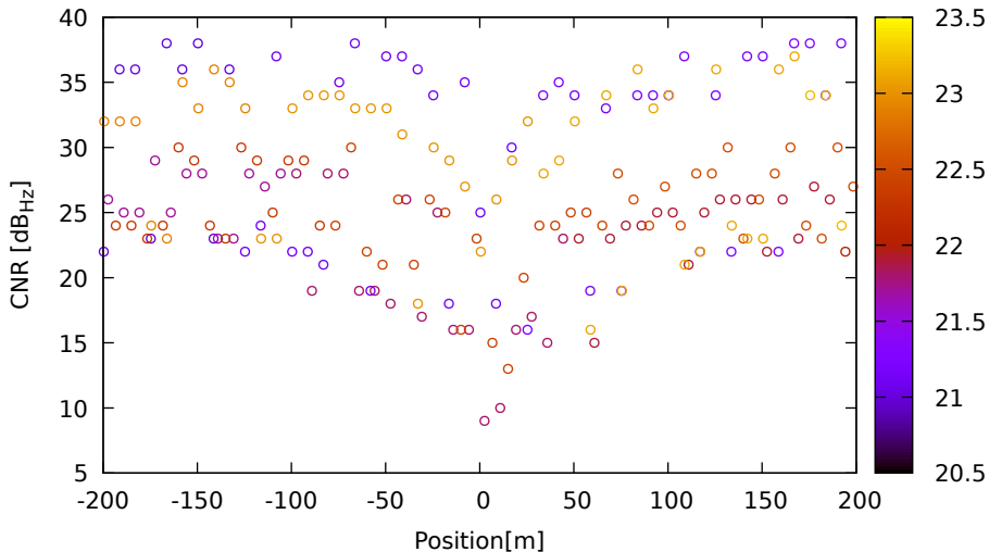
CNR vs position for C33 (B1) on HuaweiP40 - DOY 263 jam. 1
