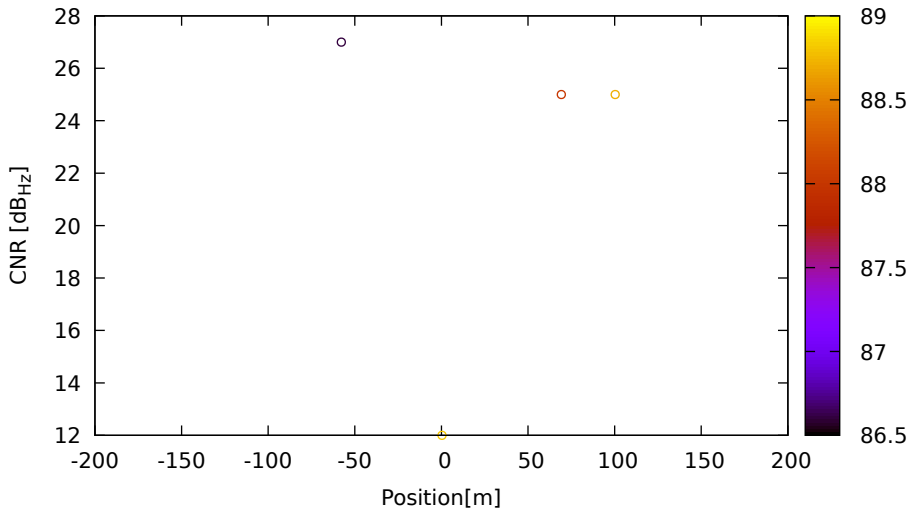
CNR vs position for E12 (E5a) on HuaweiP40 - DOY 263 jam. 1
