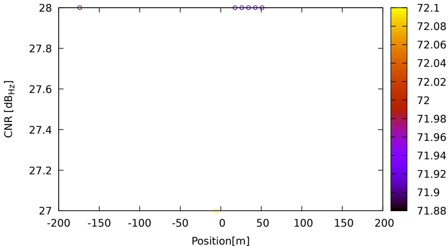
CNR vs position for E19 (E5a) on HuaweiP40 - DOY 263 jam. 3
