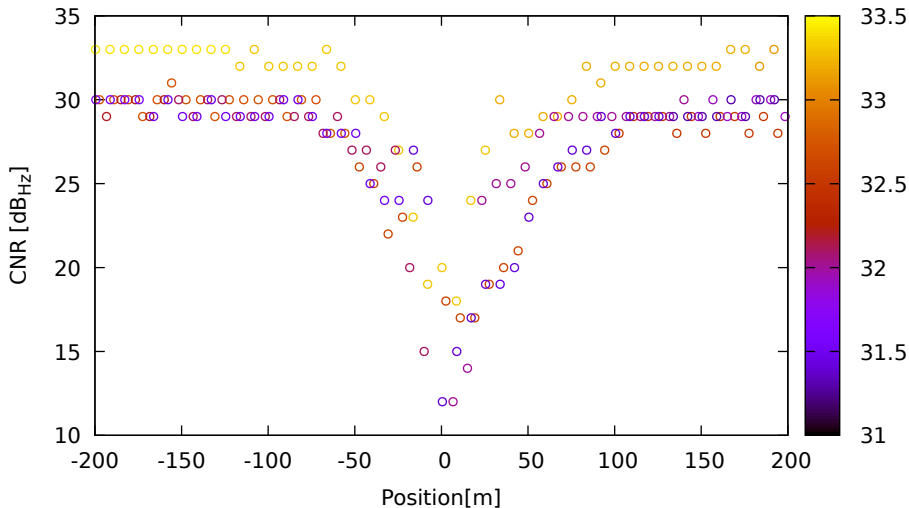
CNR vs position for E33 (E1) on HuaweiP40 - DOY 263 jam. 1
