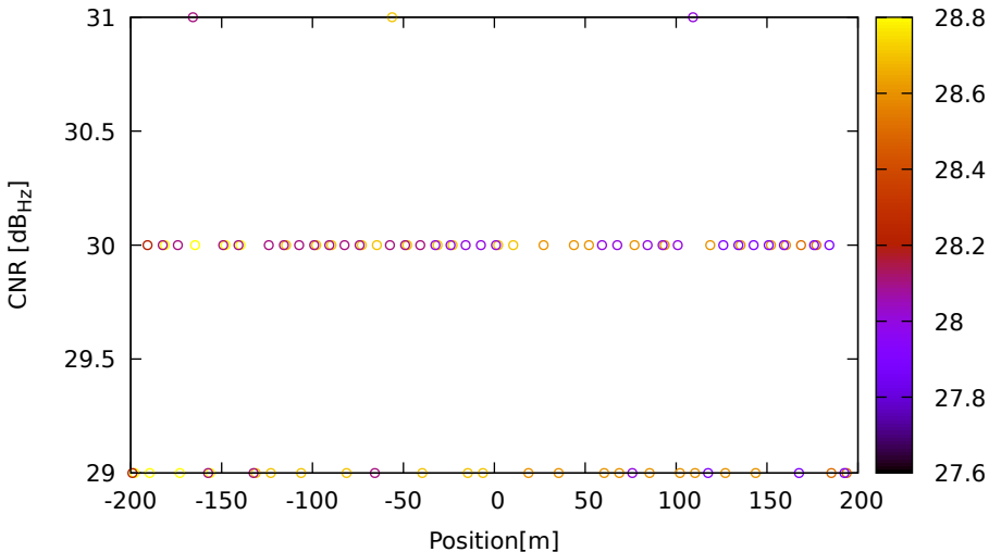
CNR vs position for E33 (E1) on HuaweiP40 - DOY 263 jam. 3
