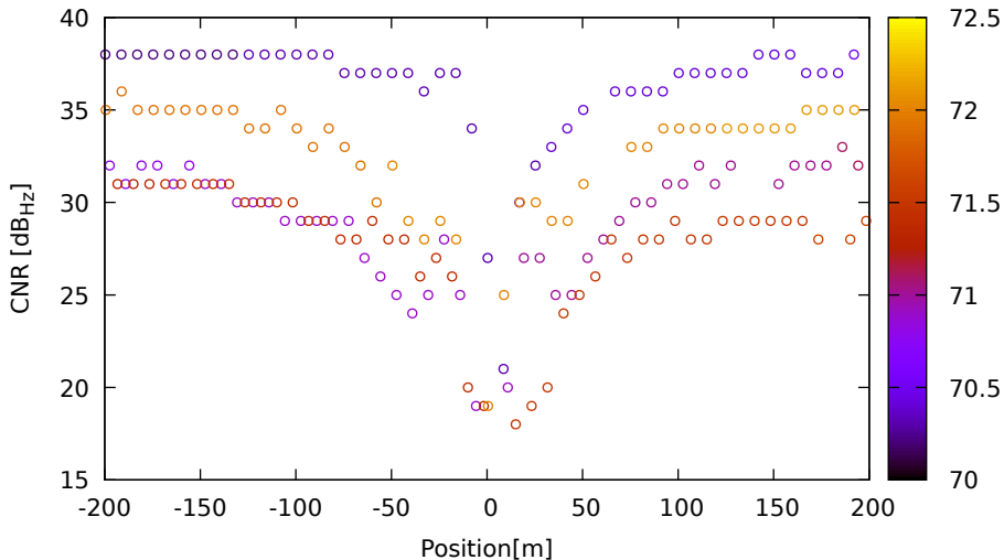
CNR vs position for G03 (L1) on HuaweiP40 - DOY 263 jam. 1
