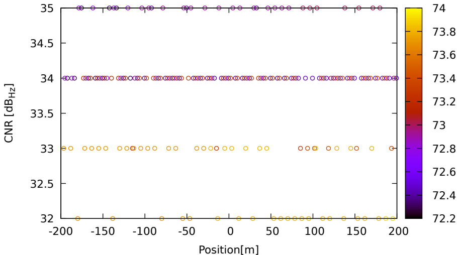
CNR vs position for G03 (L5) on HuaweiP40 - DOY 263 jam. 2
