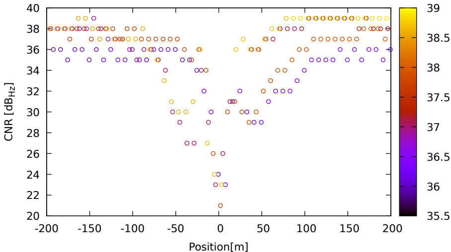
CNR vs position for G04 (L1) on HuaweiP40 - DOY 263 jam. 2
