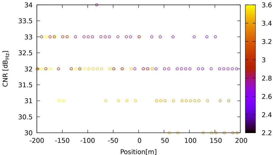
CNR vs position for G08 (L5) on HuaweiP40 - DOY 263 jam. 3
