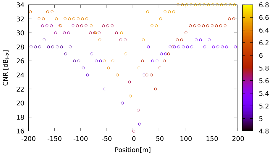
CNR vs position for G09 (L1) on HuaweiP40 - DOY 263 jam. 2
