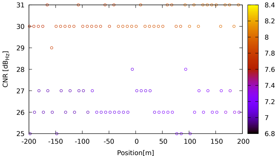
CNR vs position for G09 (L5) on HuaweiP40 - DOY 263 jam. 3
