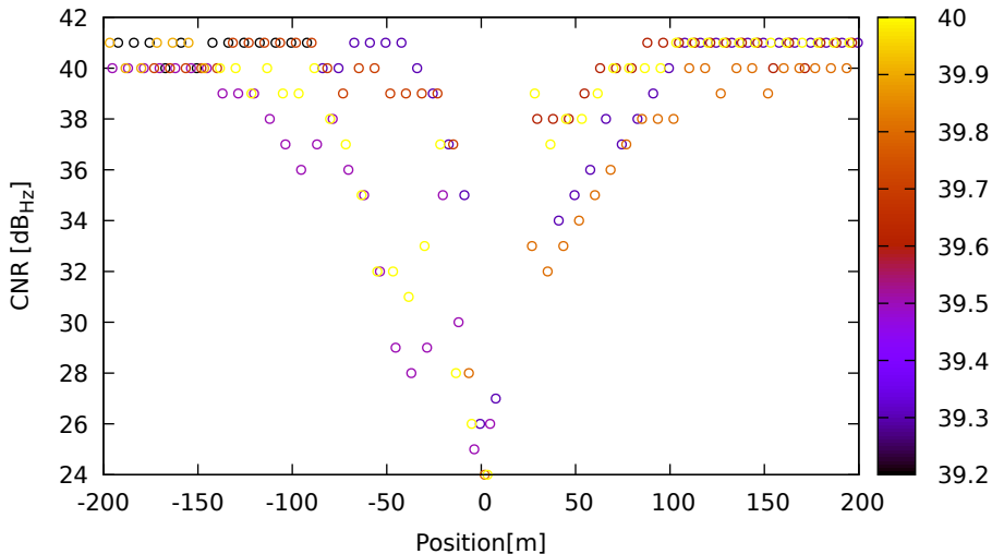
CNR vs position for G17 (L1) on HuaweiP40 - DOY 263 jam. 2
