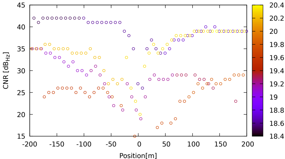
CNR vs position for G19 (L1) on HuaweiP40 - DOY 263 jam. 2
