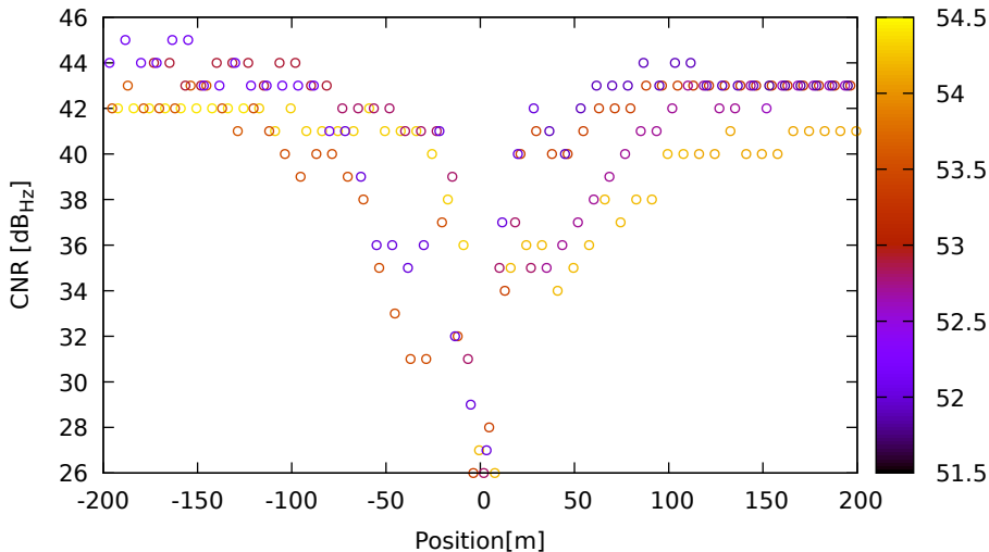
CNR vs position for G21 (L1) on HuaweiP40 - DOY 263 jam. 2
