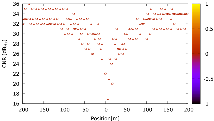
CNR vs position for G28 (L1) on HuaweiP40 - DOY 263 jam. 1
