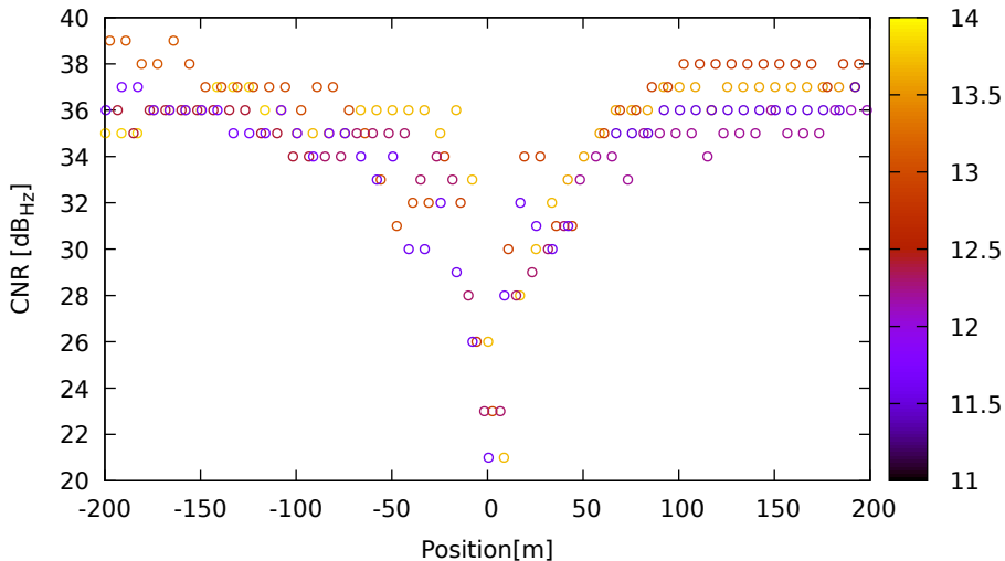
CNR vs position for G32 (L1) on HuaweiP40 - DOY 263 jam. 1
