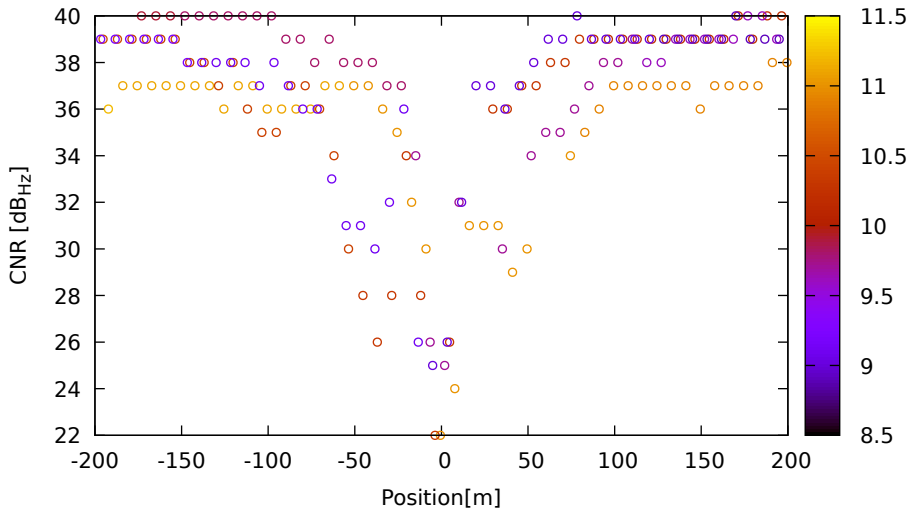
CNR vs position for G32 (L1) on HuaweiP40 - DOY 263 jam. 2
