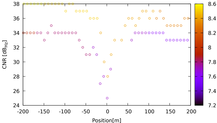
CNR vs position for G32 (L1) on HuaweiP40 - DOY 263 jam. 3
